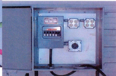
Typical vendor's Rental panel (Has 4 individual 20 amp Receptacles, 1 50 amp receptacle)
