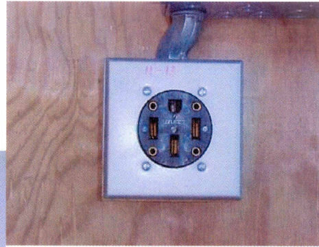
Same receptacle As on right (only 50 amp receptacle Configuration accepted).
