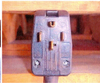
Typical 50 amp male plug (note; amps and voltage. This is the only 50 amp plug accepted).
