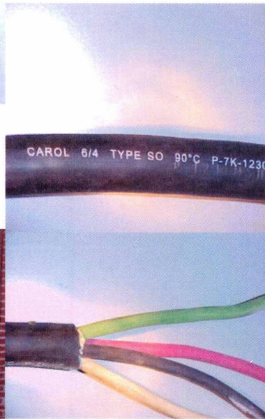
This is the electrical cord excepted at River fest. note; cord has to be a minimum of 8 gauge, 4 conductor
